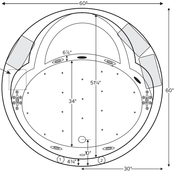
Numbered areas on tub deck represent possible locations to install cleaning systems, faucets and other fixtures. Shown with Air Massage and Ultra Whirlpool Package.
