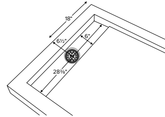
Hidden drain cover is removable for access.
